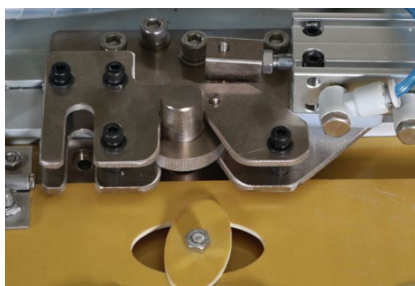
Automatic Clamping and Framing Device
